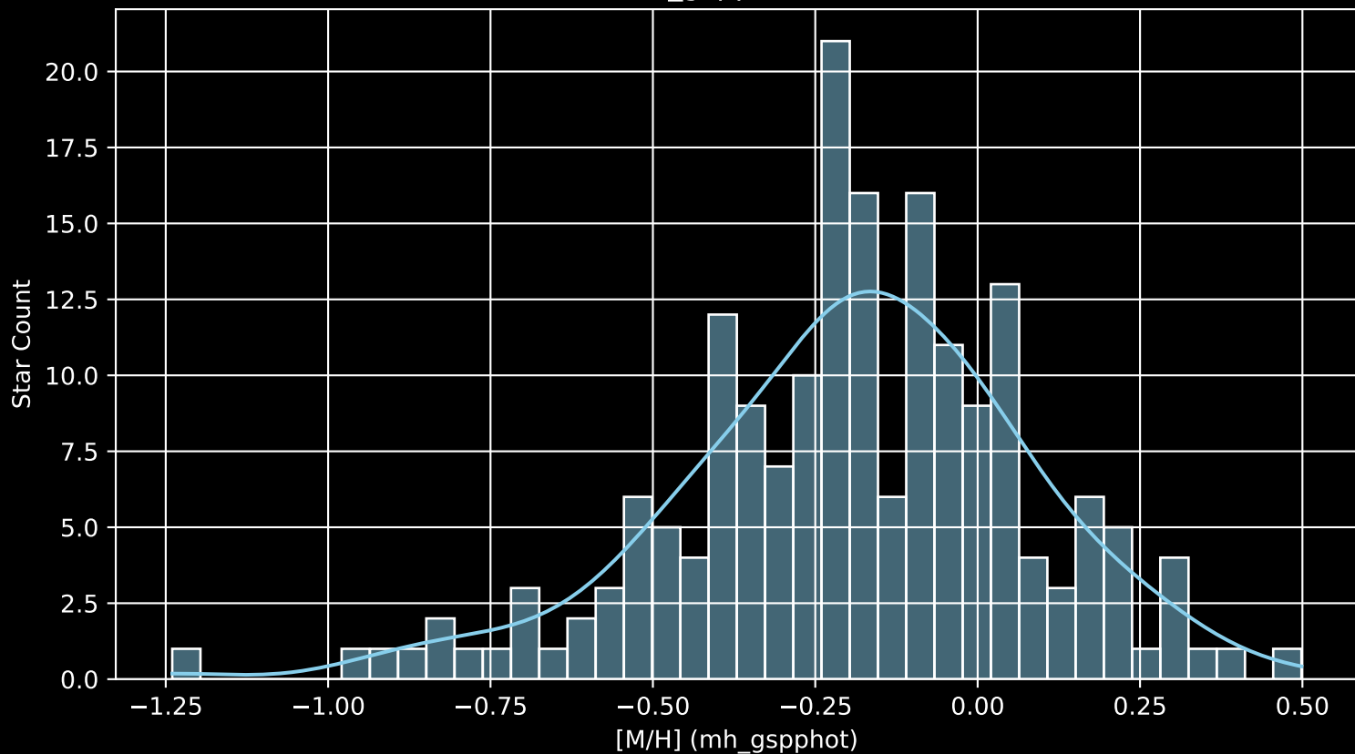
APOGEE DR17 Field: [185+27_MGA [M/H] (mh_gspphot) (n= 188)
