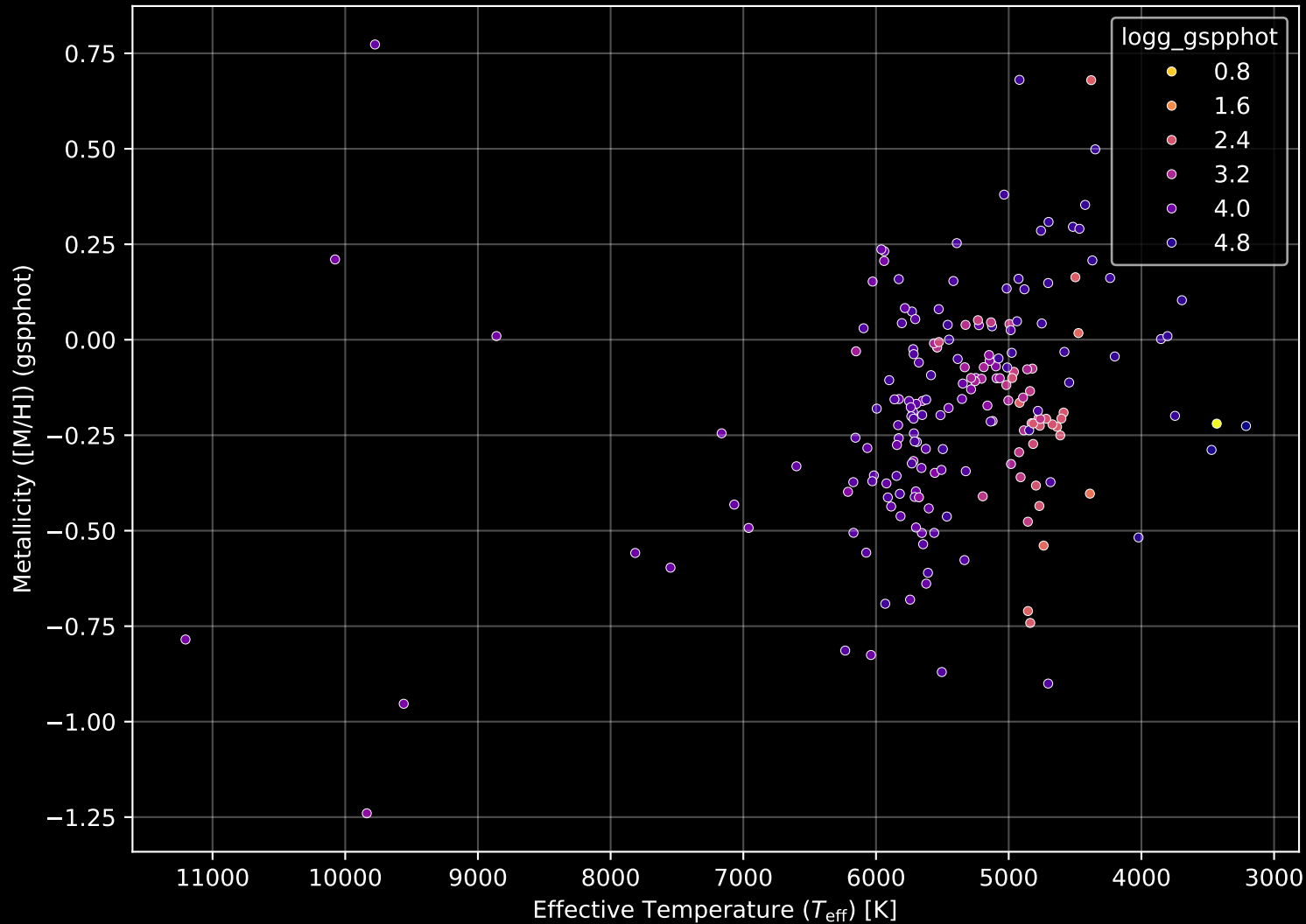
APOGEE DR17 Field: [185+27_MGA] Stellar Population Parameters (n= 191)
