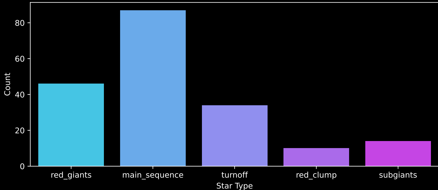
APOGEE DR17 Field: [185+27_MGA] Count plot of Star Type
