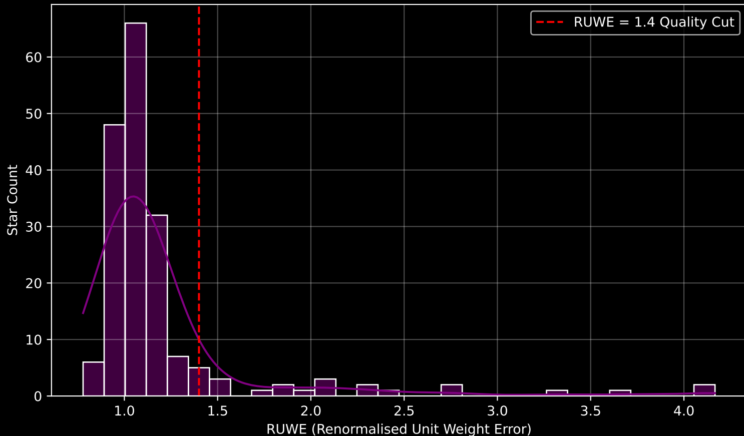
GAPOGEE DR17 Field [185+27_MGA] RUWE Distribution (n= 183)
