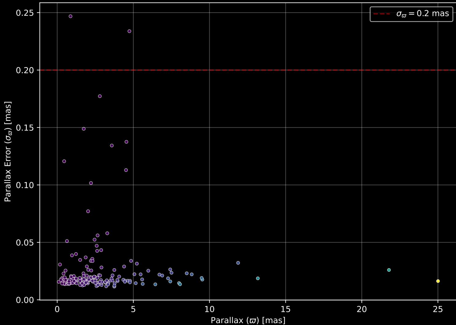
APOGEE DR17 Field: [185+27_MGA] Parallax Quality (n= 191)
