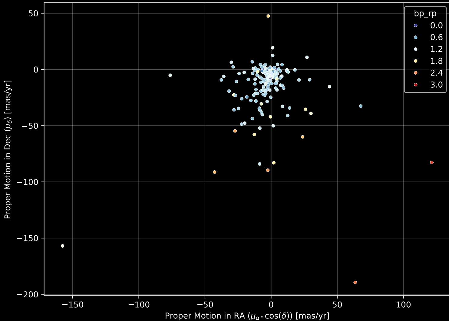
APOGEE DR17 Field: [185+27_MGA] Proper Motion Diagram (n= 191)
