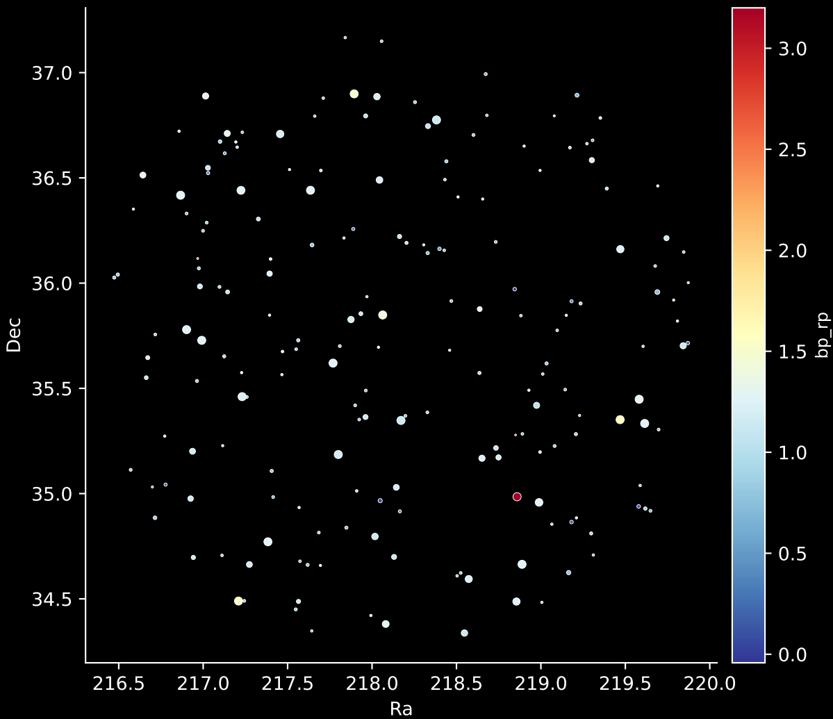
APOGEE DR17 Field: [185+27_MGA] Stars: 191
