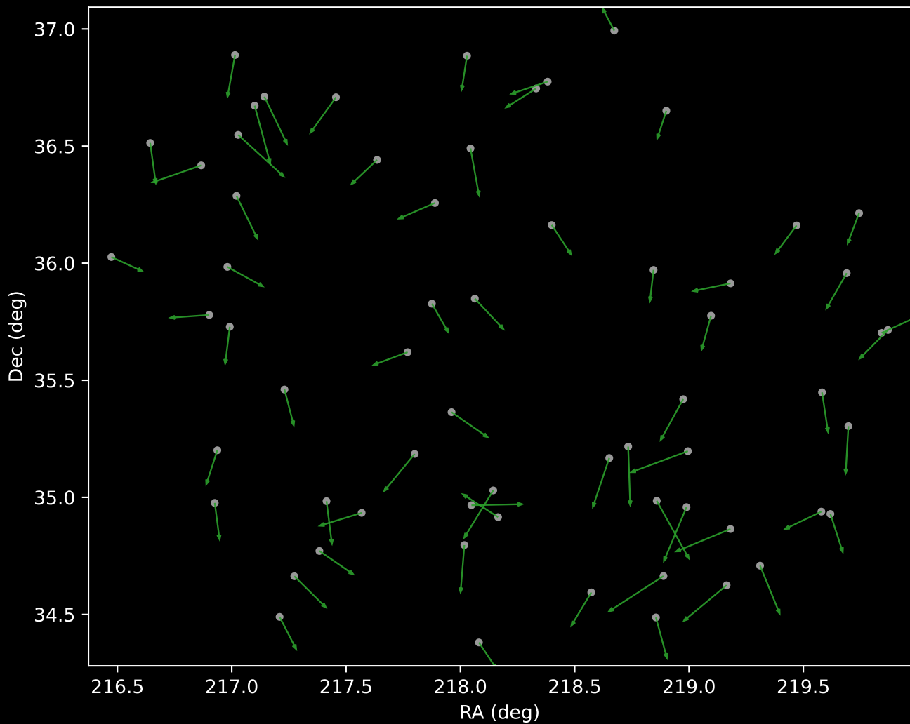
APOGEE DR17 Cluster 4 Proper Motion Vectors (n=63)
